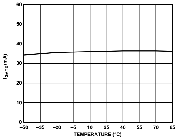
Figure 13. I_{GATE} (FCL, Sink) vs. Temperature ( V_{GATE} = 2 V )
